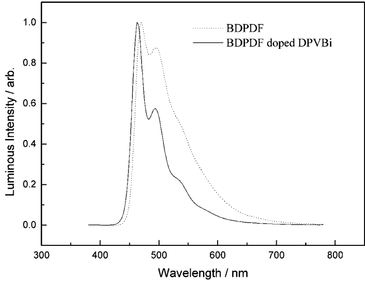
FIGURE 4 EL spectra of devices using BDPDF as an emissive layer (dot line) and doped into DPVBi (solid line).
