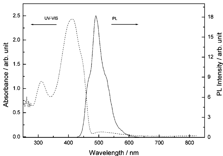
FIGURE 1 UV-visible (dot line) and photoluminescence (solid line) spectra of BDPDF thin film on quartz substrate (excitation wavelength 410 nm).
