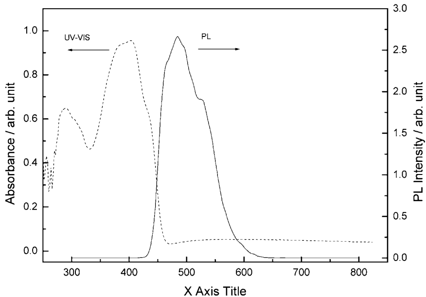
FIGURE 2 UV-visible (dot line) and photoluminescence (solid line) spectra of BECDF thin film on quartz substrate (excitation wavelength 404 nm).
