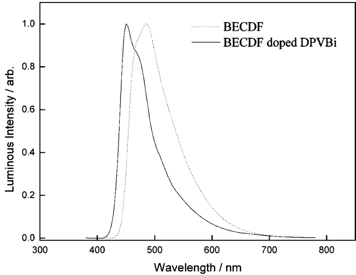
FIGURE 5 EL spectra of devices using BECDF as an emissive layer (dot line) and doped into DPVBi (solid line).
