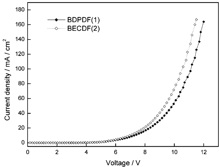
FIGURE 3 Current-voltage (I-V) characteristics of undoped EL devices.
